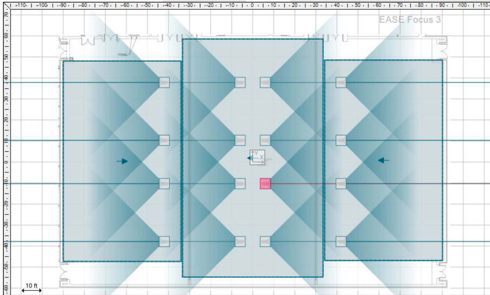
Speaker Layout, top view
