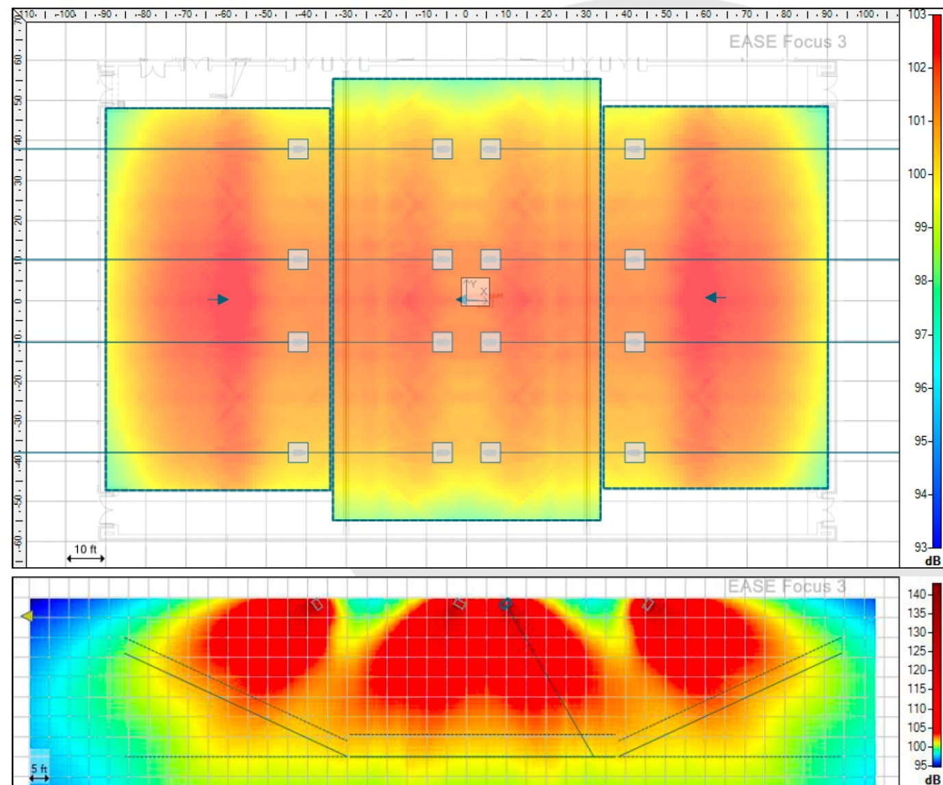
A-Weighted SPL coverage, top view and end view
