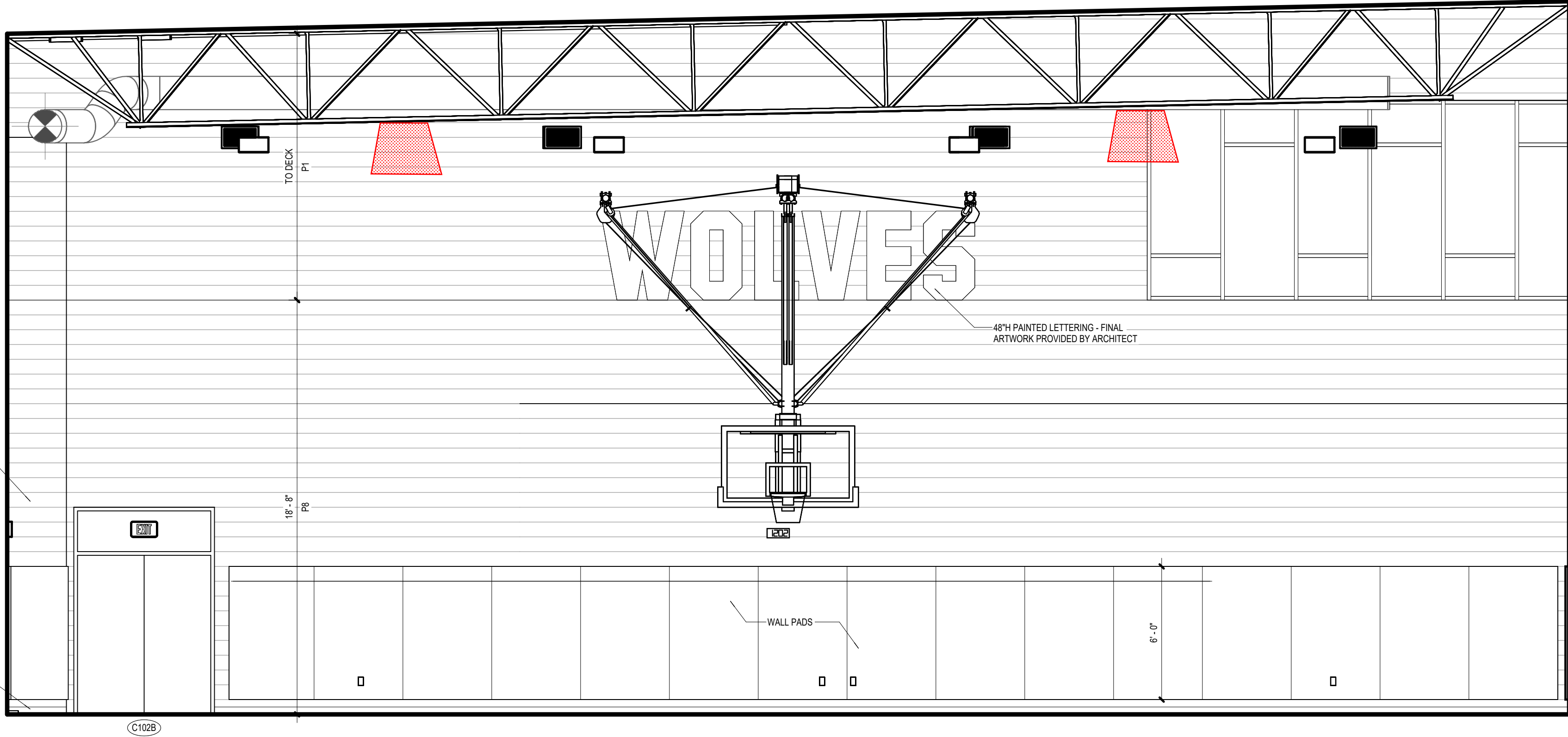
1 A8.12 C102 AUXILIARY GYMNASIUM NORTH 1/4" = 1'-0"
