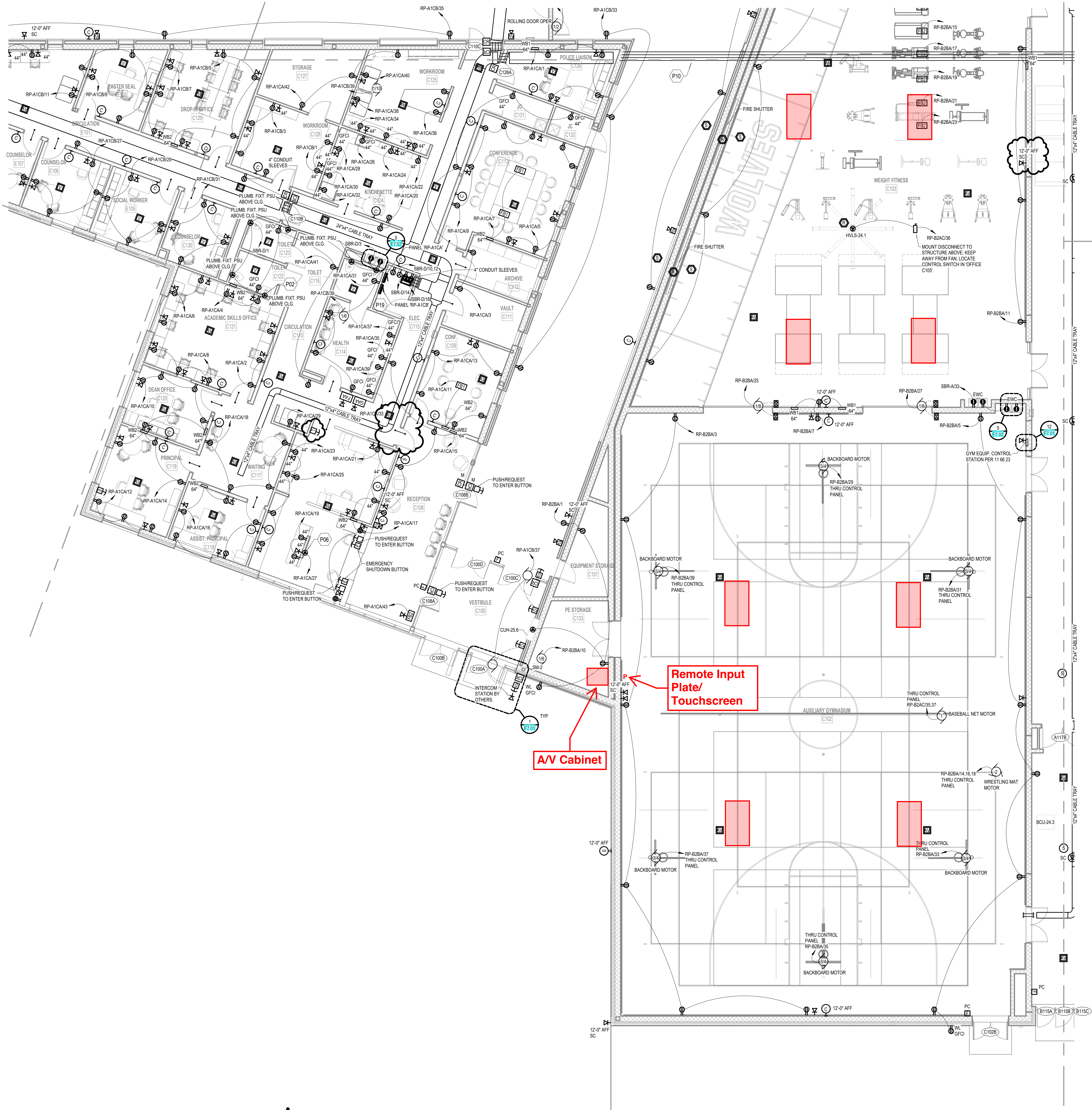
UNIT 'C' FIRST FLOOR POWER & COMMUNICATIONS PLAN
