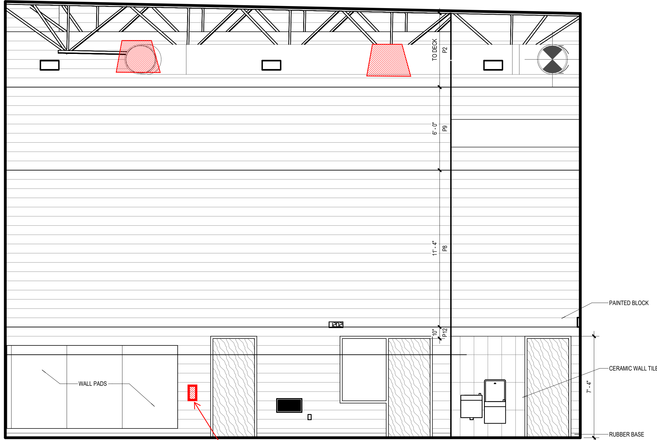
4 A8.12 C103 WEIGHT FITNESS SOUTH 1/4" = 1'-0"
