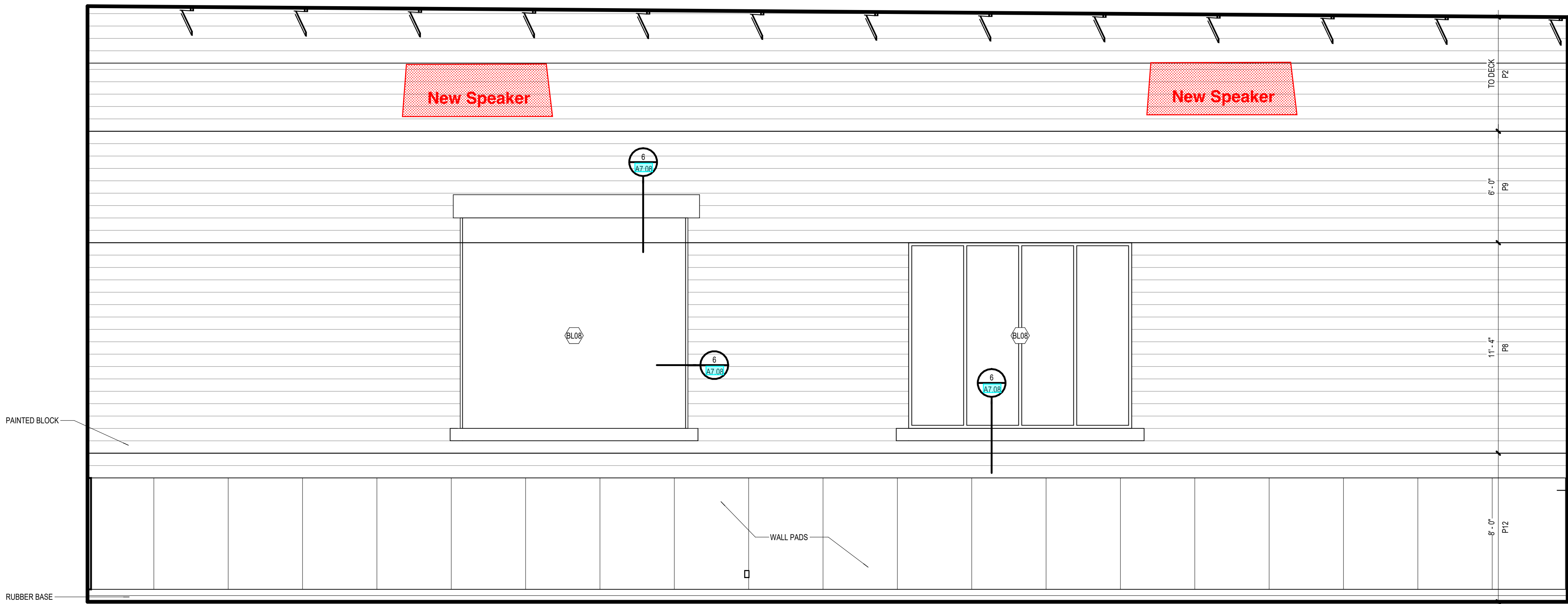
5 A8.12 C103 WEIGHT FITNESS EAST 1/4" = 1'-0"
