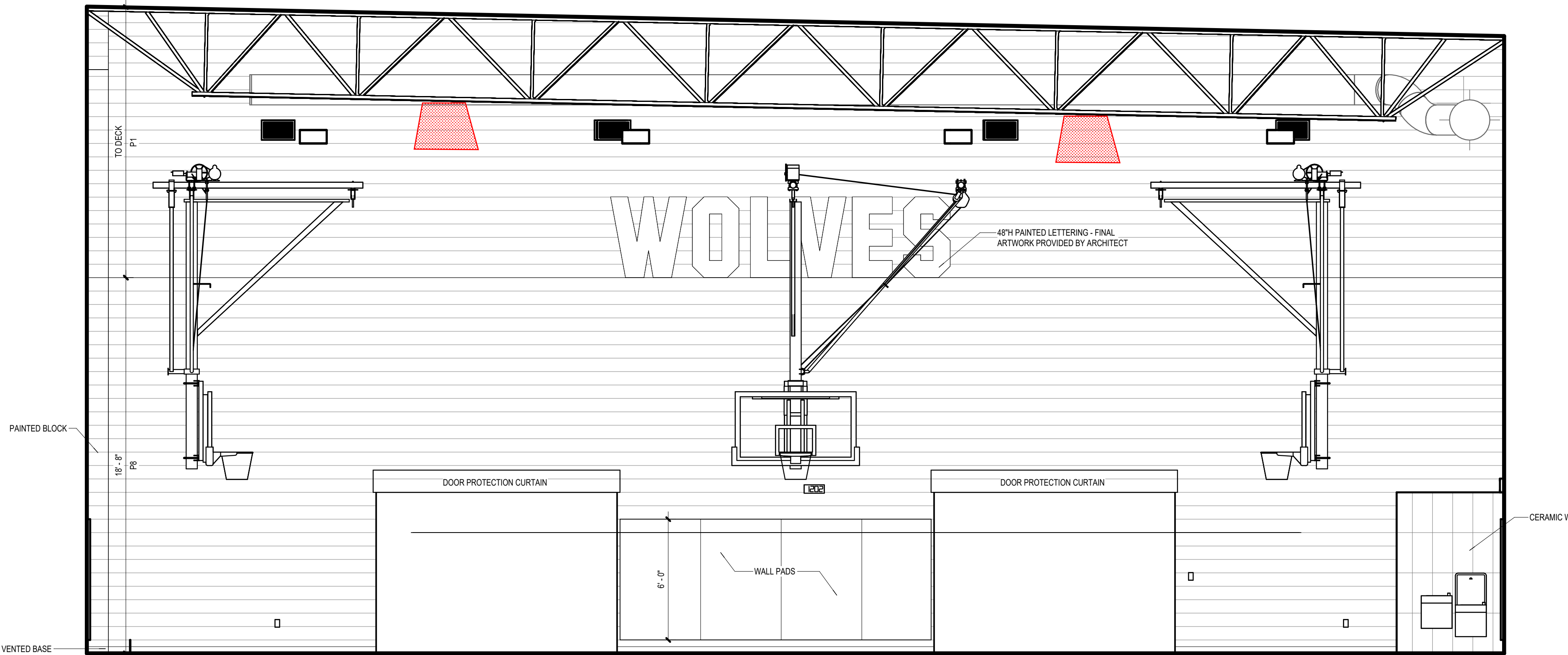
2 A8.11 C102 AUXILIARY GYMNASIUM SOUTH 1/4" = 1'-0"
