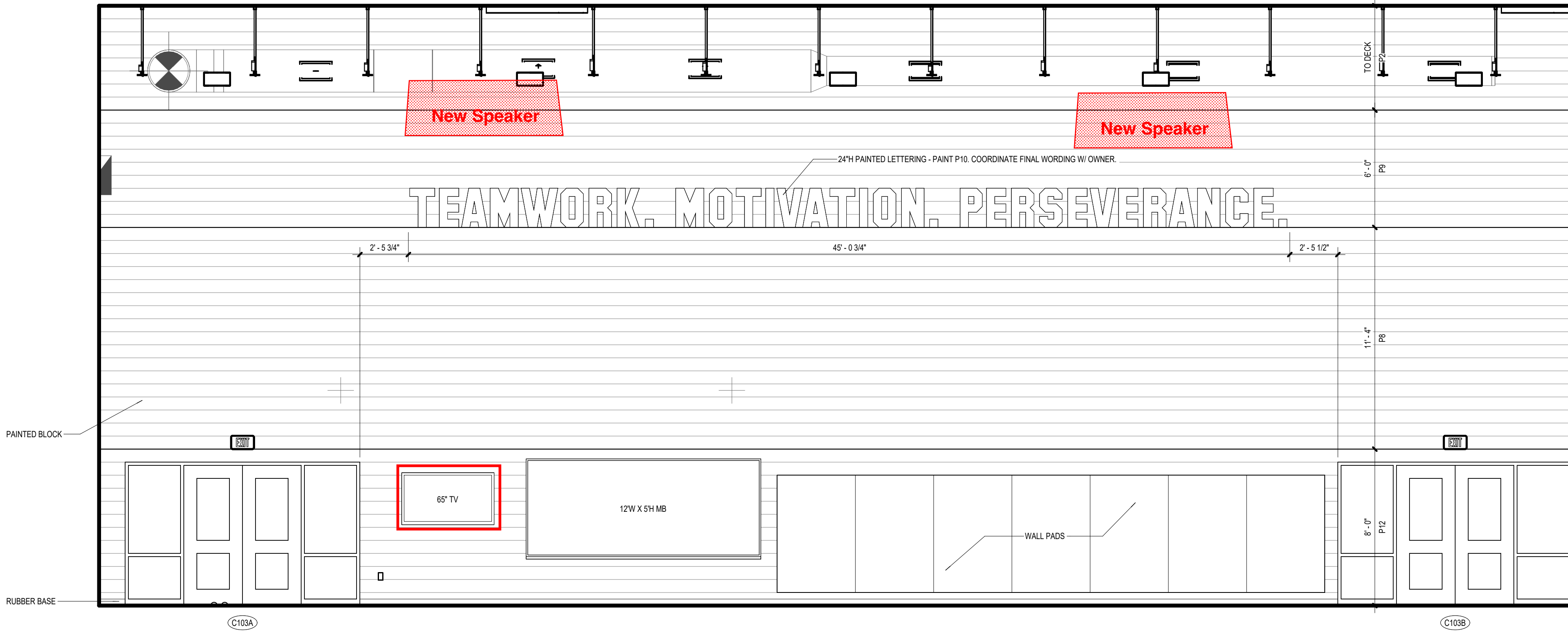
3 A8.12 C103 WEIGHT FITNESS WEST 1/4" = 1'-0"
