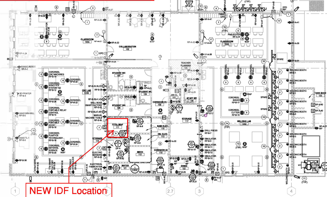
LEVEL 1 POWER AND AUXILIARY SYSTEMS PLAN SCALE: 1/8" = 1'-0"
