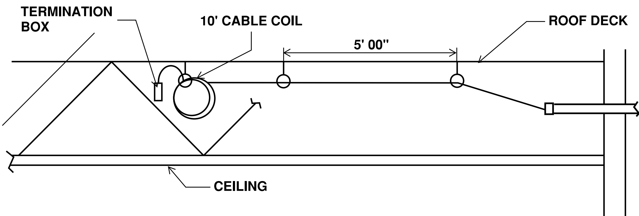
TYP 3 - SURFACE MOUNTED POWER & DATA OUTLET DETAIL NOT TO SCALE
