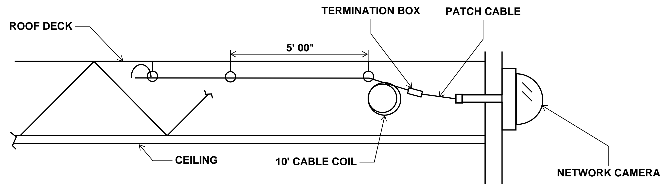
TYP 1 - EXTERIOR MOUNTED NETWORK CAMERA NOT TO SCALE
