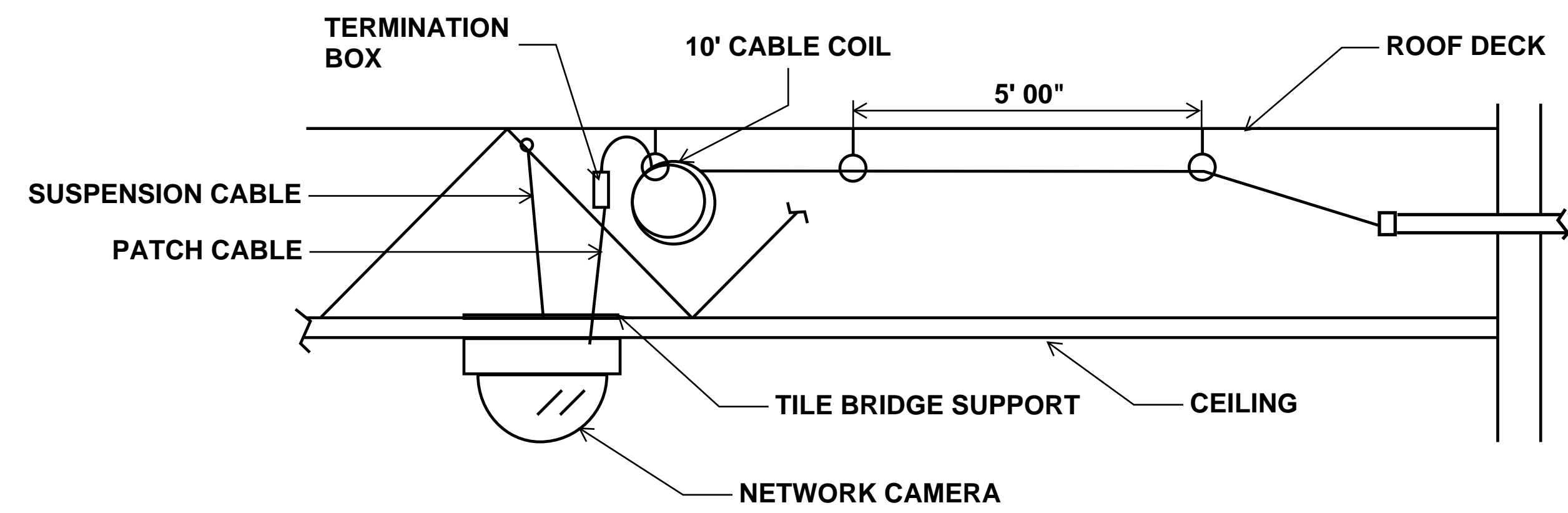
TYP 2 - INTERIOR MOUNTED NETWORK CAMERA NOT TO SCALE
