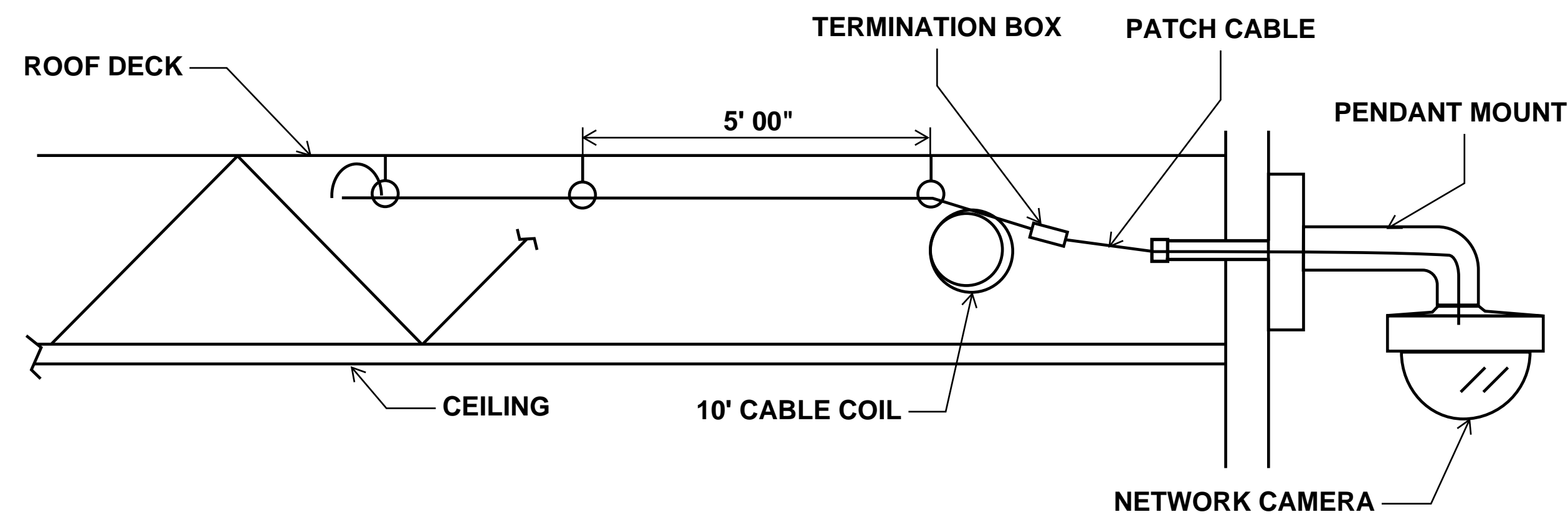
TYP 3 - EXTERIOR MOUNTED NETWORK CAMERA WITH PENDANT NOT TO SCALE
